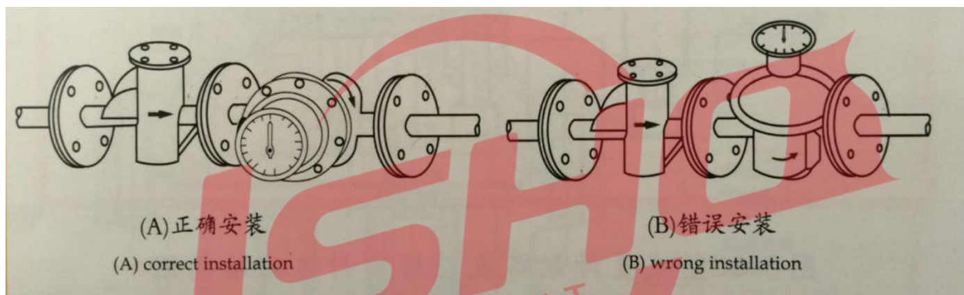
图4 安装姿势 Picture 4 Installation position
